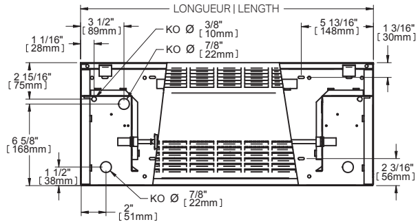
DEVANT | FRONT
