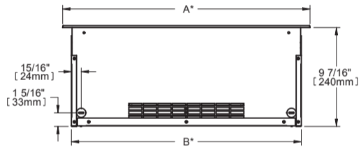
DEVANT | FRONT
