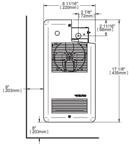
DEVANT | FRONT
