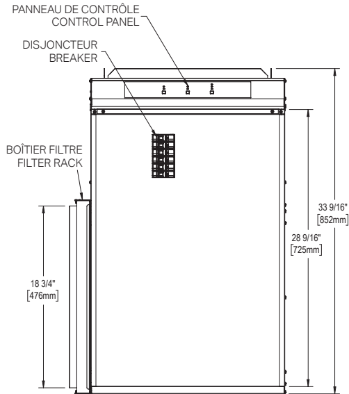
DEVANT | FRONT
