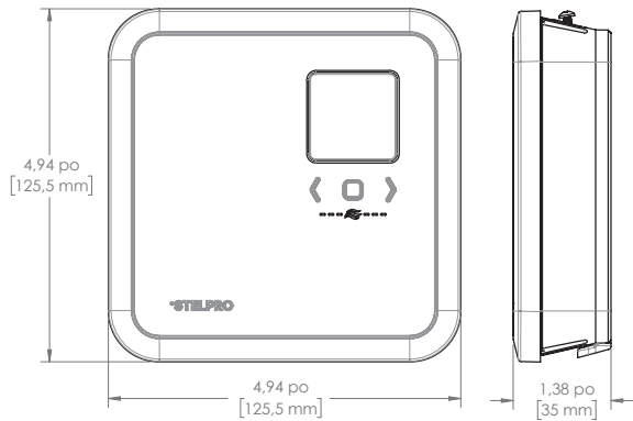
DEVANT | FRONT
