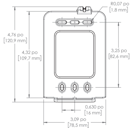
PLAQUE DE MONTAGE | MOUNTING PLATE
