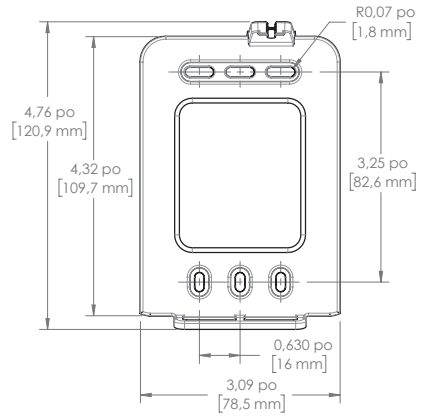
PLAQUE DE MONTAGE | MOUNTING PLATE
