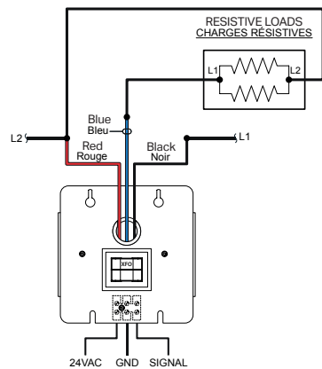
BRANCHEMENT / CONNECTION | CCT-25-1-C2-T240
