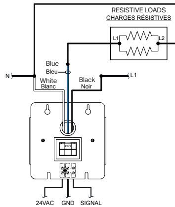
BRANCHEMENT / CONNECTION | CCT-25-1-C2-T347
