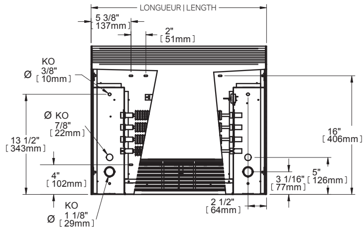
DEVANT | FRONT
