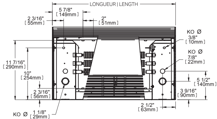
DEVANT | FRONT
