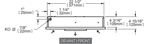
DRR - installation encastrée / recessed
