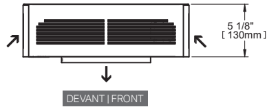
DRI - installation en surface / surface mounted
