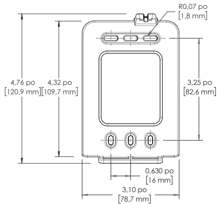
PLAQUE DE MONTAGE | MOUNTING PLATE
