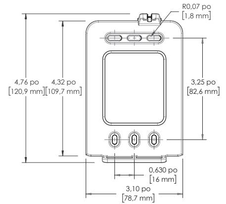
PLAQUE DE MONTAGE | MOUNTING PLATE
